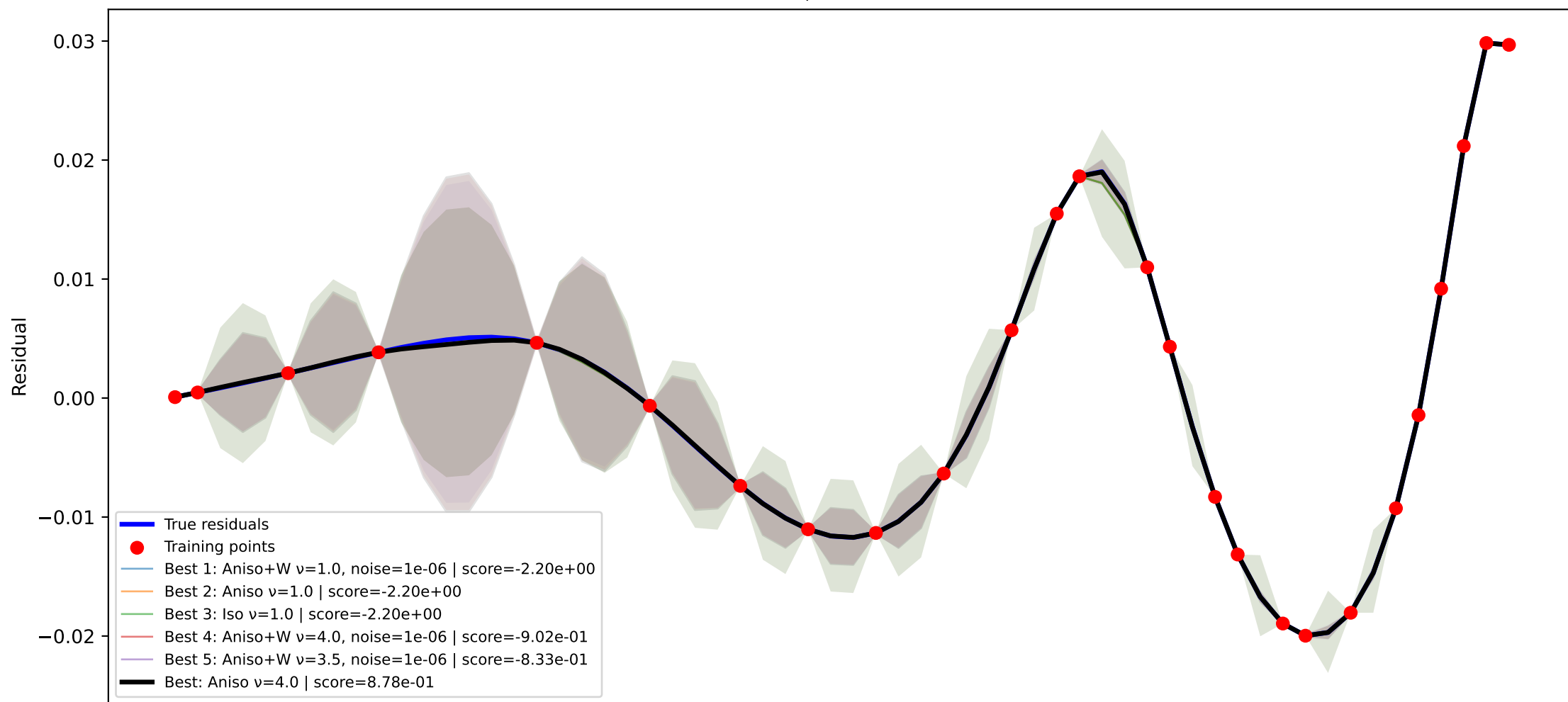
GPR kernel comparison node=12 RMSE=9.385e-05, train RMSE=3.608e-11
